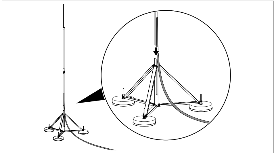
Fig. 45: Inserting the air-termination rod in the tripod stand
