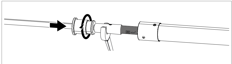
Fig. 29: Screwing the air-termination rod to the connection element
