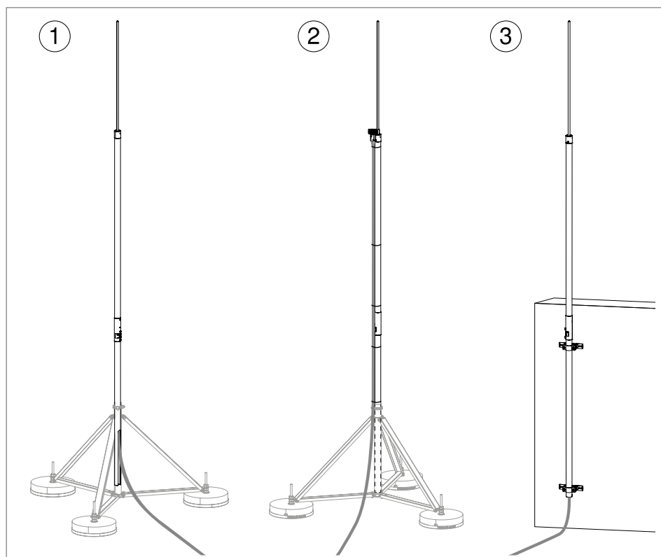
Fig. 4: Three air-termination rod types (without potential connection)
