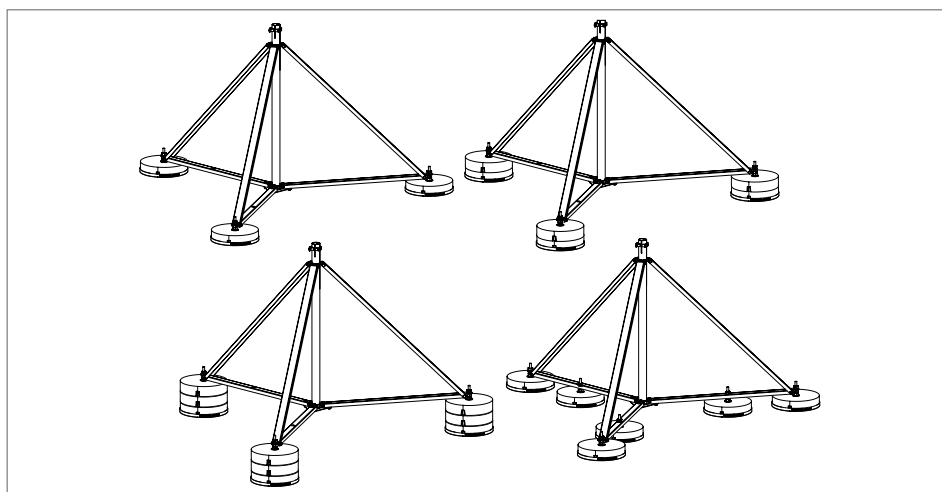
Fig. 8: Increasing the stand weight by stacking the concrete blocks
