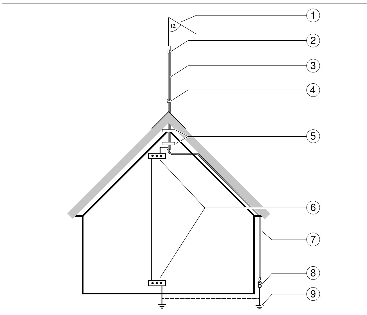
Fig. 17: Installation example: Soft-covered roof
