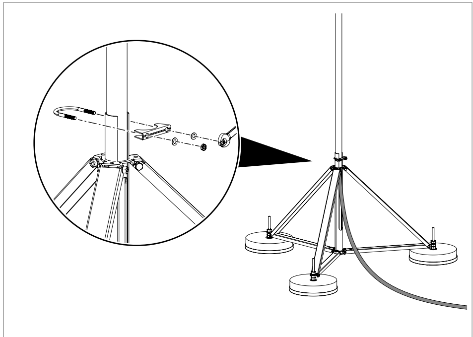
Fig. 46: Fastening the air-termination rod in the air-termination rod stand
