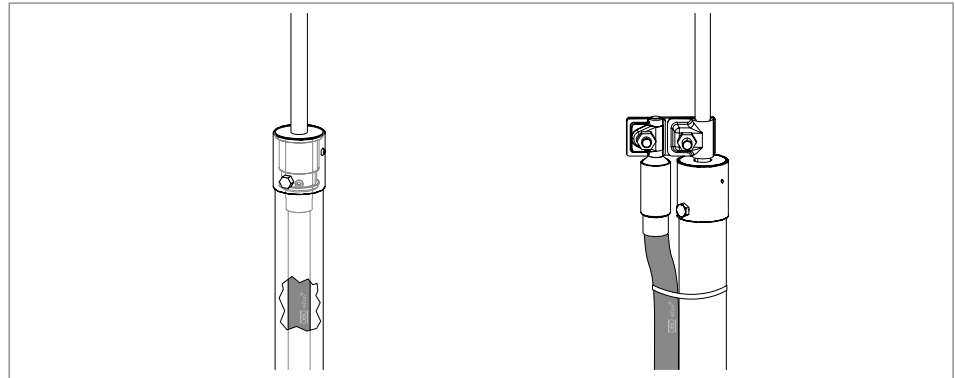
Fig. 15: One isCon® conductor for lightning protection class II/I
