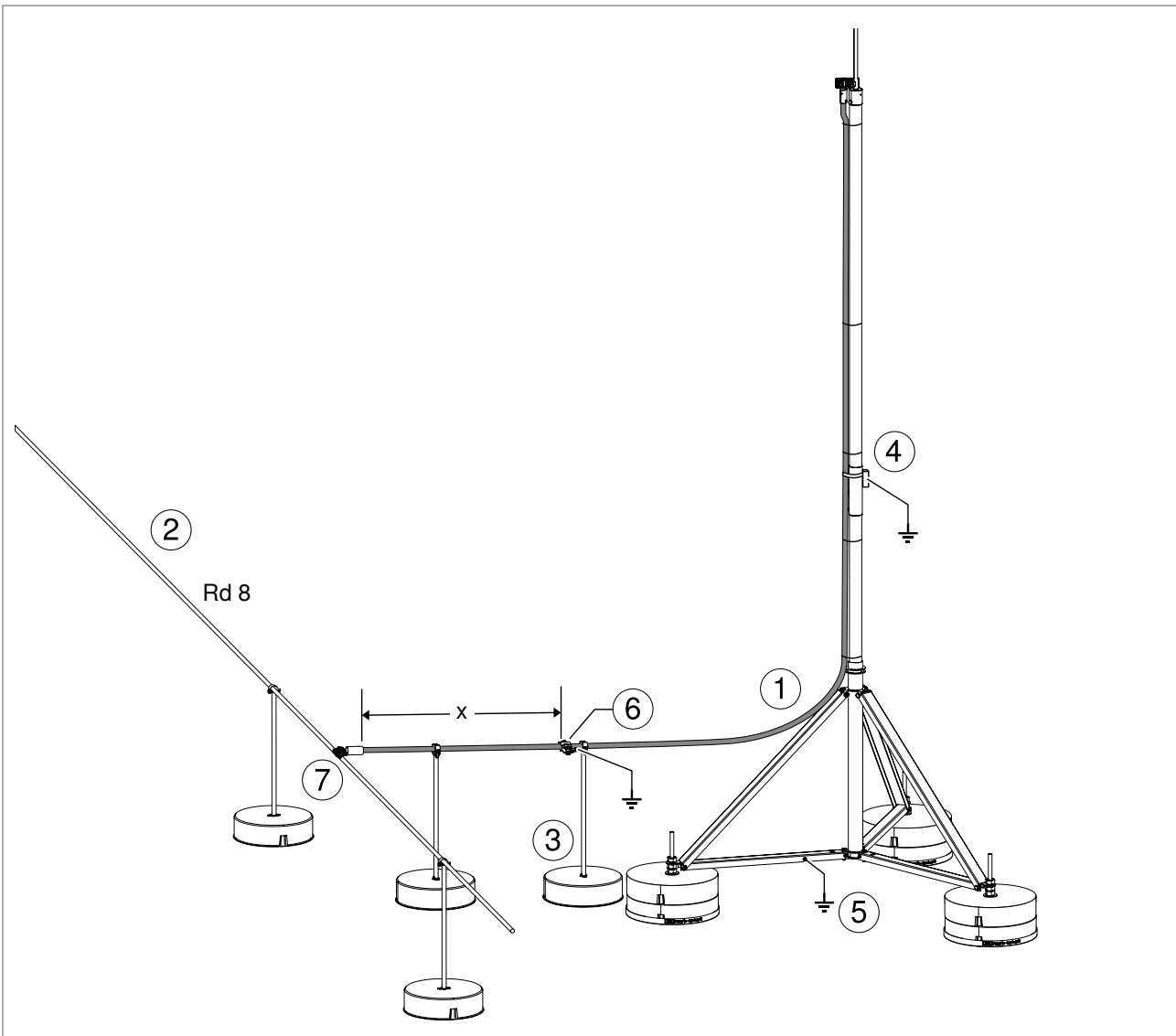
Fig. 61: isCon® conductor connected to stand-off ring conductor
