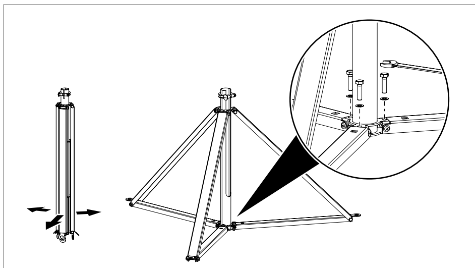
Fig. 42: Unfolding and fixing the tripod stand
